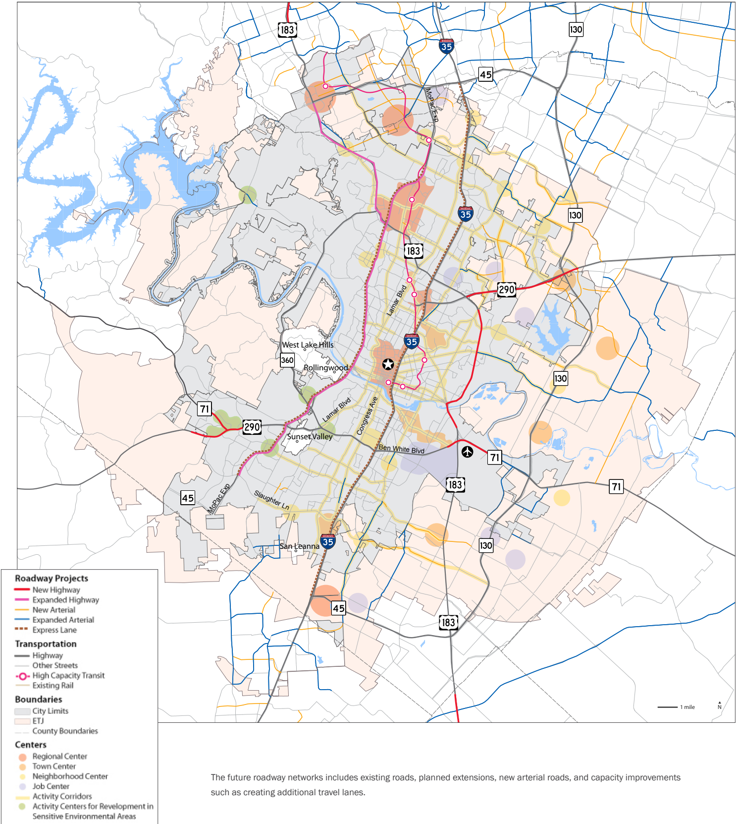
Figure 4.4 Roadway Networks
